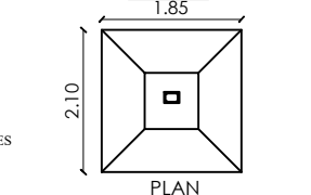
FOUNDATION DETAILS
