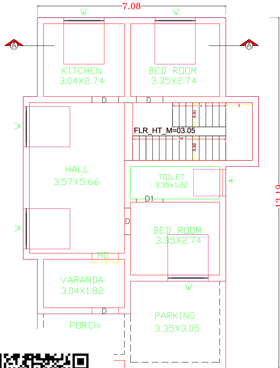
FLOOR PLAN
