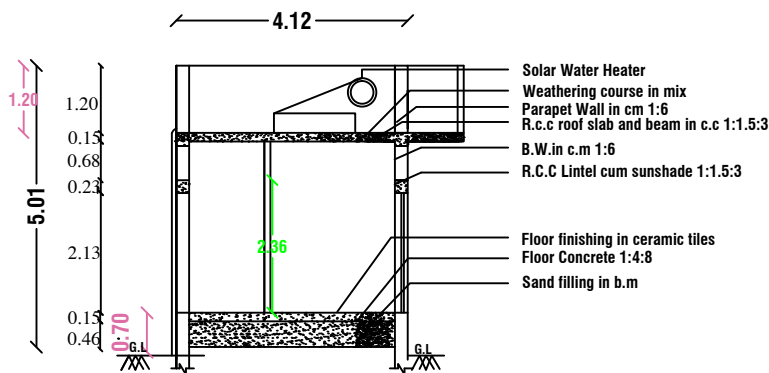
SECTION - "AB "
