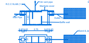
SEPTIC TANK & TRENCH
