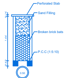
WATER COLLECTION WELL
