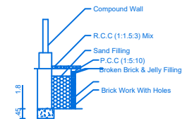
RAIN WATER HARVEST DETAILS
