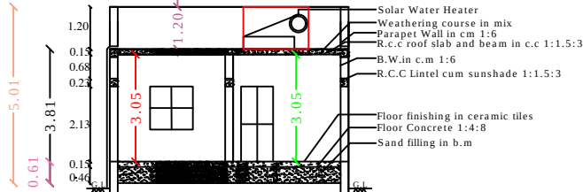
SECTION - "AB "
