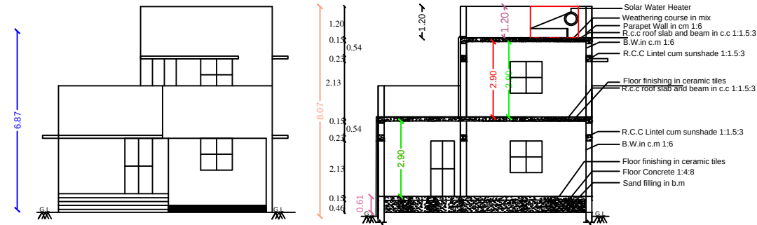
SECTION - "AB - CD"
