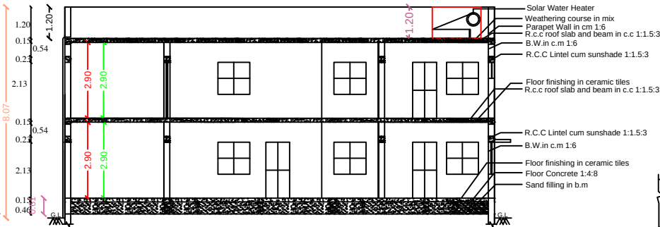
SECTION - "AB-CD"
