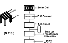
SOLAR SYSTEM FLOW DIAGRAM
