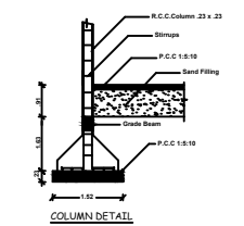
COLUMN DETAIL
