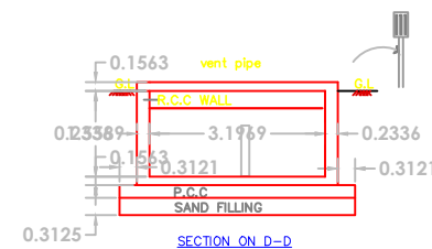
SECTION ON D-D
