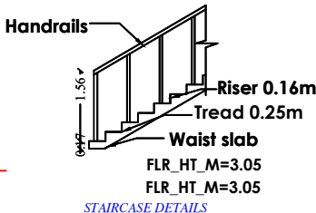
STAIRCASE DETAILS
