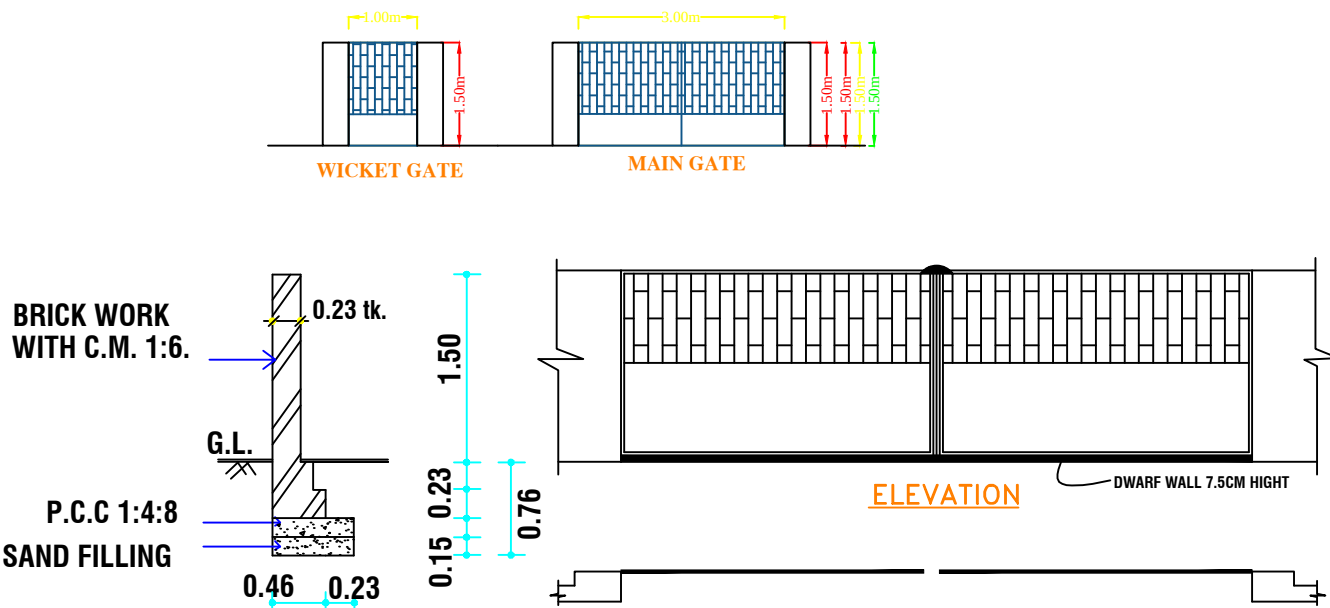
SECTION OF COMPOUND WALL
