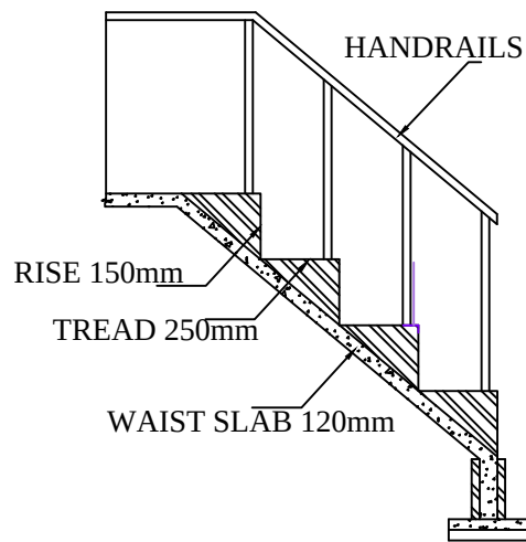
STAIRCASE DETAILS
