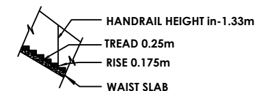
STAIRCASE DETAILS
