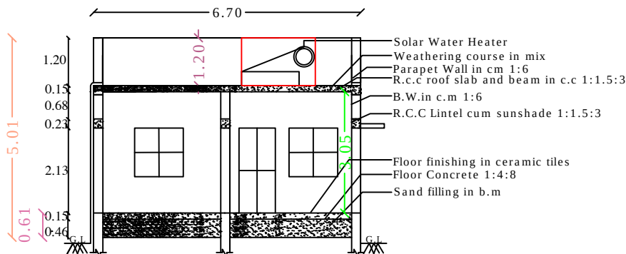
SECTION - "AB "
