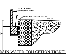
RAIN WATER COLLECTION TRENCH
