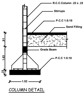
COLUMN DETAIL
