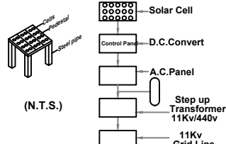
SOLAR SYSTEM FLOW DIAGRAM
