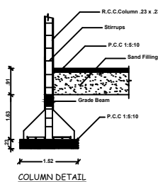
COLUMN DETAIL
