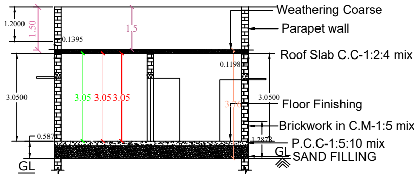
CROSS SECTION ON XX
