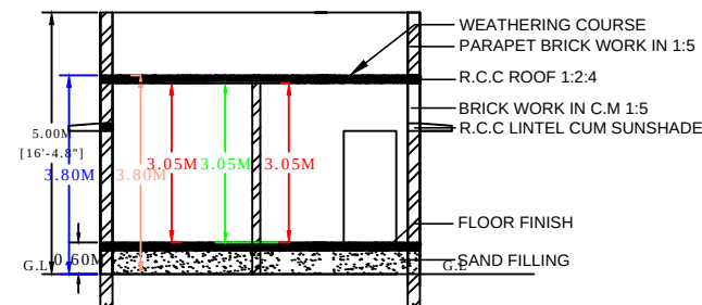
SECTION ON XX
