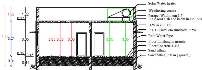
SECTION - "AB"
