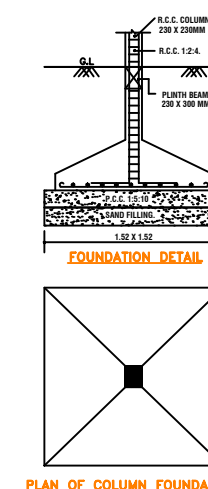
FOUNDATION DETAIL
