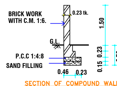
SECTION OF COMPOUND WALL
