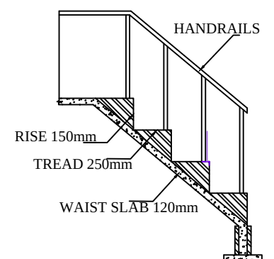
STAIRCASE DETAILS
