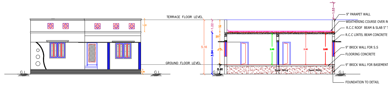
FRONT ELEVATION
