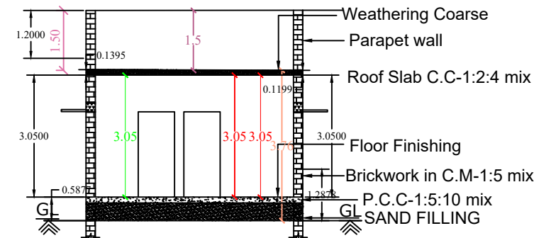
CROSS SECTION ON XX
