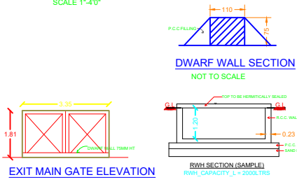
EXIT MAIN GATE ELEVATION
