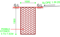
SECTION OF PEBBLE TRENCH SCALE : 1" = 100
