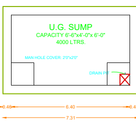
SUMP DETAIL SCALE 1"=2'-0"
