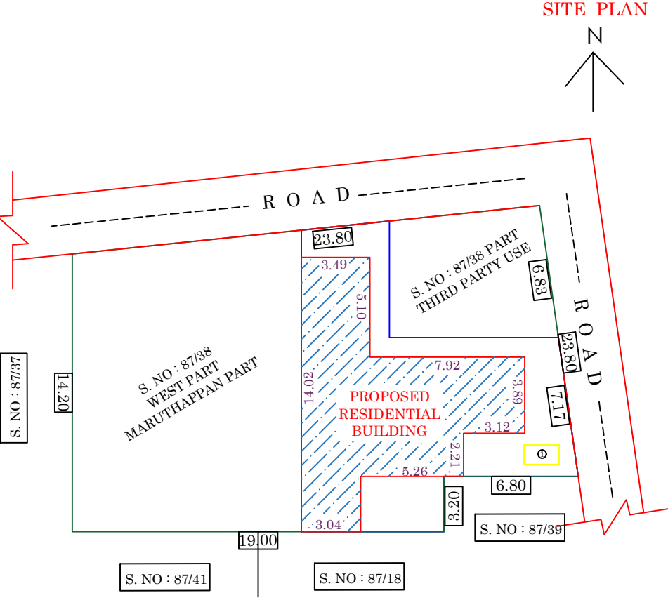
SITE PLAN
