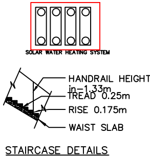
STAIRCASE DETAILS
