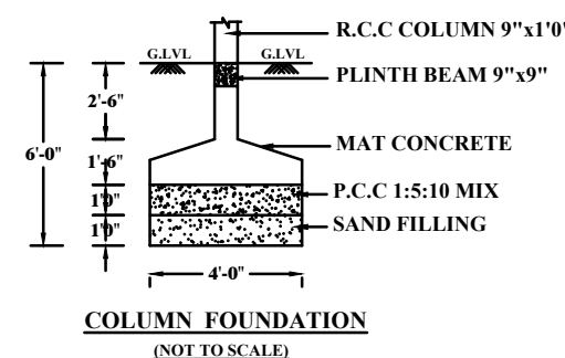
COLUMN FOUNDATION (NOT TO SCALE)
