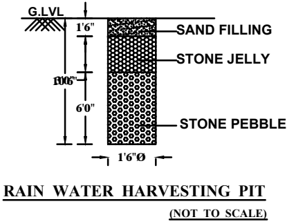
RAIN WATER HARVESTING PIT (NOT TO SCALE)
