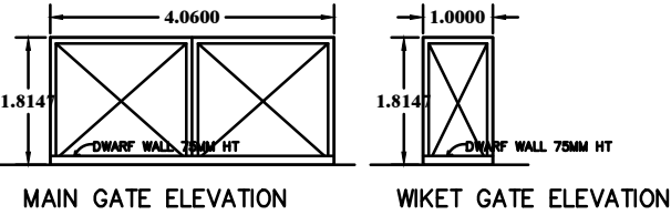
MAIN GATE ELEVATION WIKET GATE ELEVATION
