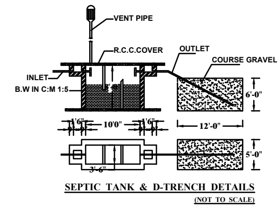
SEPTIC TANK & D-TRENCH DETAILS (NOT TO SCALE)
