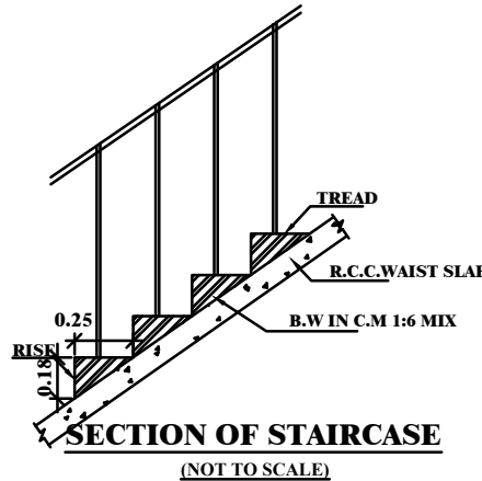
SECTION OF STAIRCASE (NOT TO SCALE)
