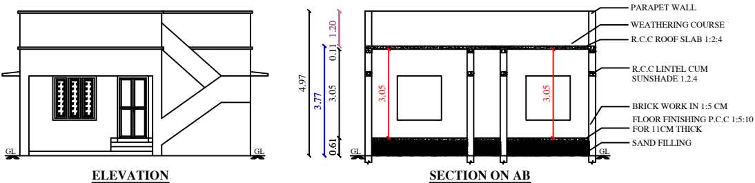
SECTION ON AB
