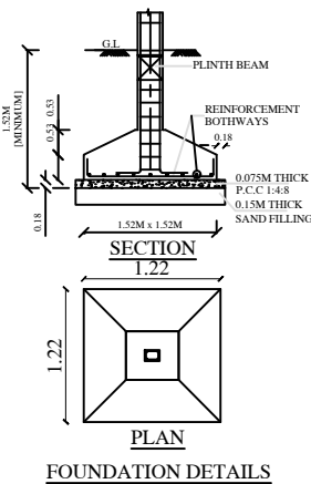
FOUNDATION DETAILS
