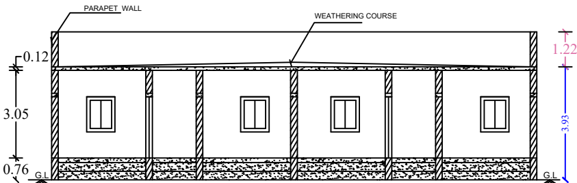
Section on-"AA"
