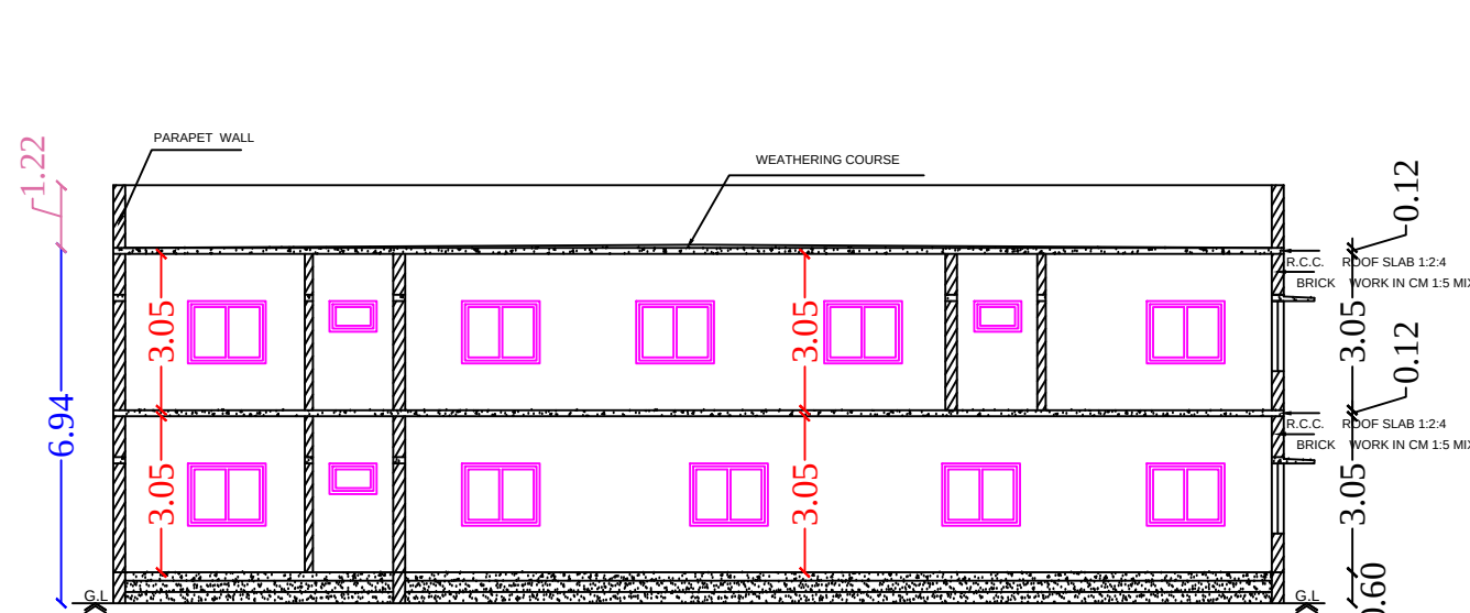
Section on-"AA"
