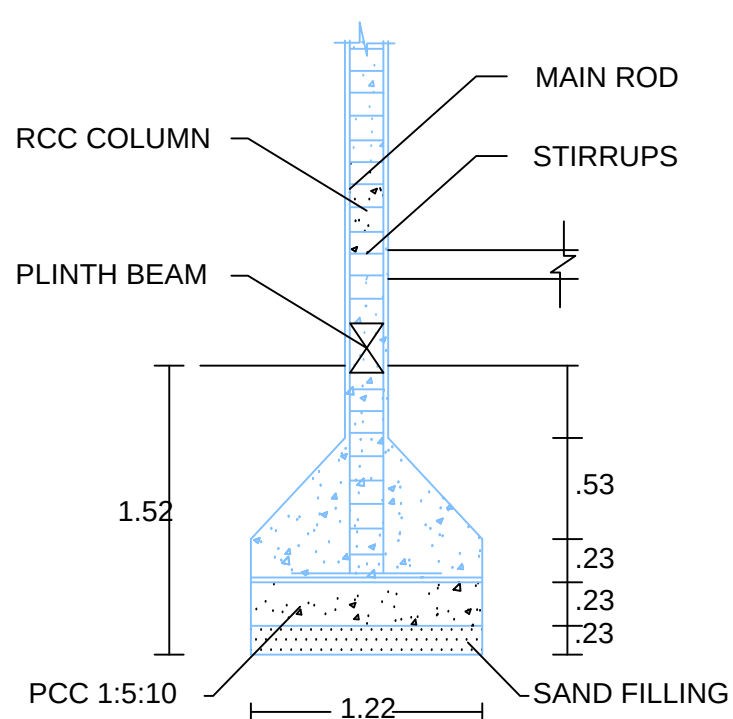
COLUMN DETAILS
