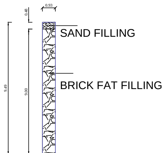
DETAILS OF PERCOLATION PIT
