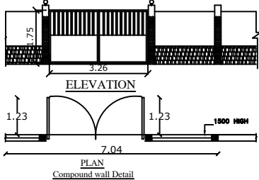
Compound wall Detail
