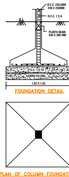
FOUNDATION DETAIL
