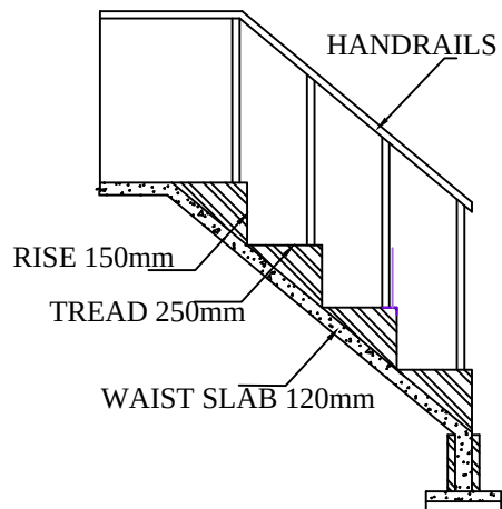
STAIRCASE DETAILS
