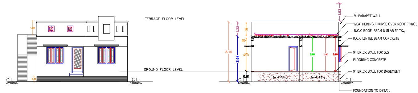
FRONT ELEVATION
