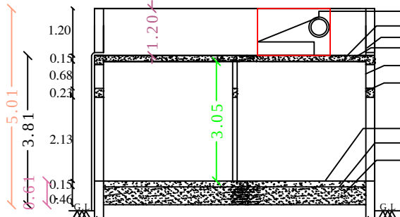
SECTION - "AB "
