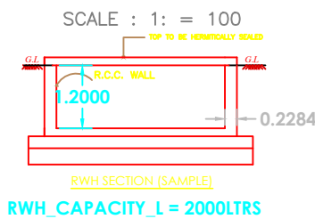
RWHP SECTION (SAMPLE)
