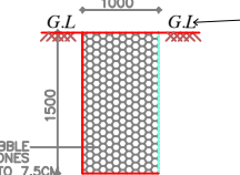
SECTION OF PEBBLE TRENCH
