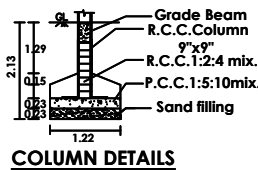
COLUMN DETAILS
