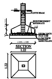
FOUNDATION DETAILS
