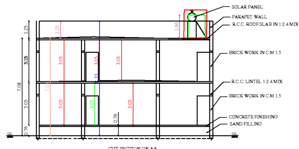
CUT SECTION OR AA
