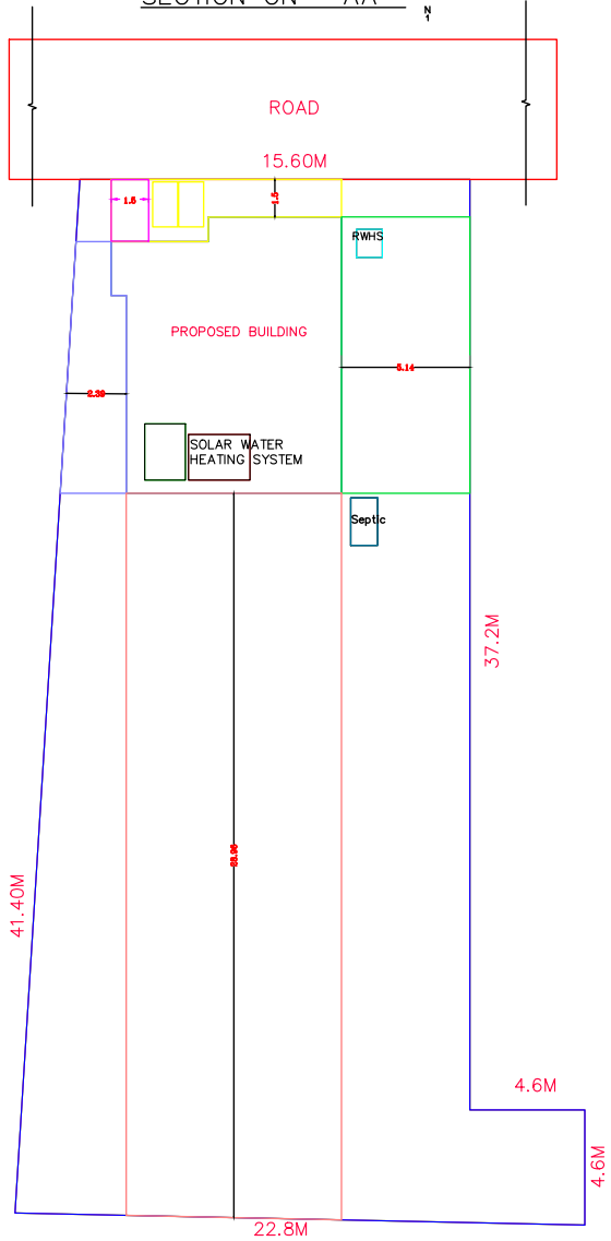
SITE PLAN
