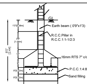
FOUNDATION DETAILS
