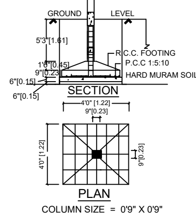
FOUNDATION DETAILS
