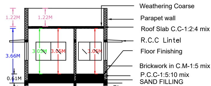
SECTION ON XX
