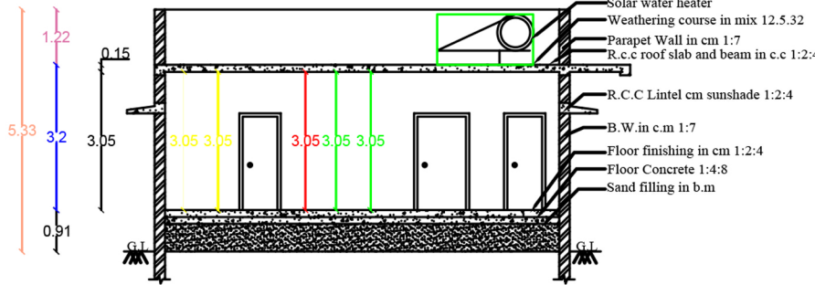
SECTION"AB,CD,EF"
