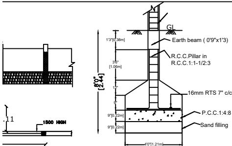
FOUNDATION DETAILS
