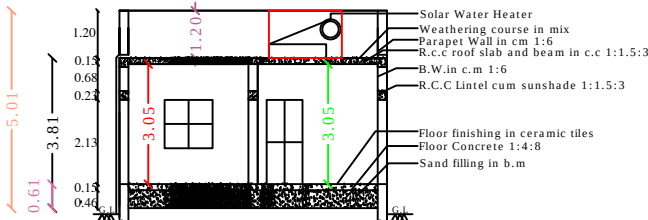
SECTION - "AB "
