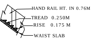
HAND RAIL HT. IN 0.76M
