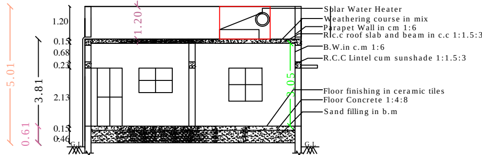
SECTION - "AB "
