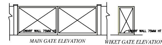
MAIN GATE ELEVATION WIKET GATE ELEVATION
