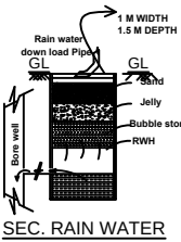
SEC. RAIN WATER HARVEST PIT
