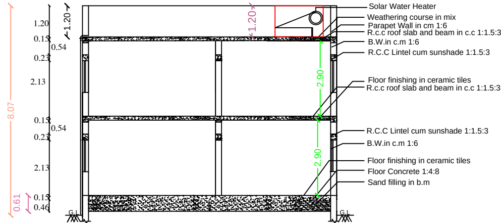
SECTION - "AB - CD"
