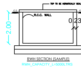
RWH SECTION (SAMPLE)
