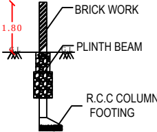
SECTION
