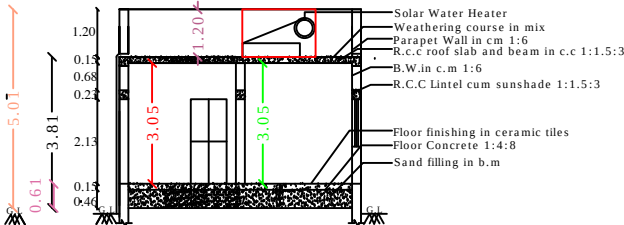
SECTION - "AB "
