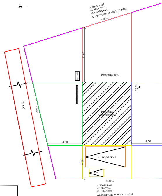
SITE PLAN
