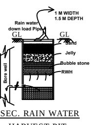
SEC. RAIN WATER HARVEST PIT
