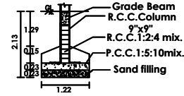
COLUMN DETAILS
