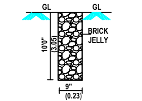
PERCOLATION PIT
