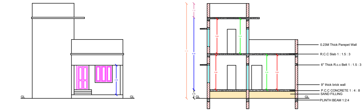
FROUNT ELEVATION
