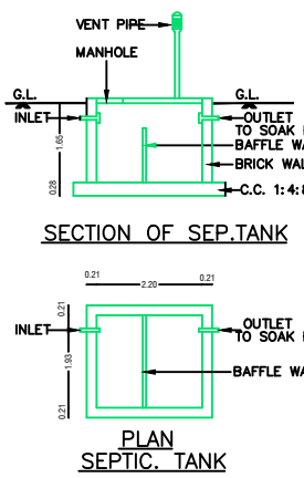
PLAN SEPTIC TANK
