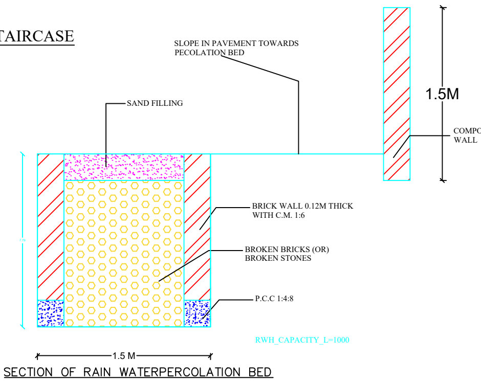
SECTION OF RAIN WATERPERCOLATION BED
