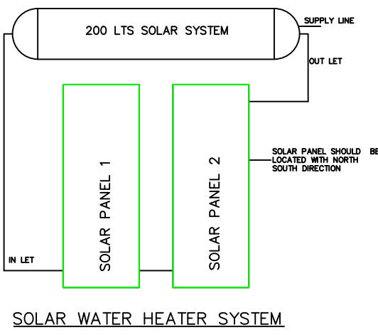
SOLAR WATER HEATER SYSTEM
