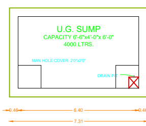
SUMP DETAIL SCALE 1"=4'-0"
