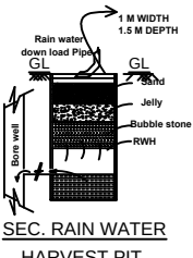
SEC. RAIN WATER HARVEST PIT
