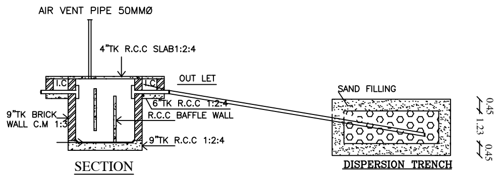
SECTION
