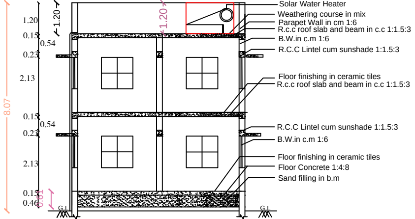
SECTION - "AB - CD"
