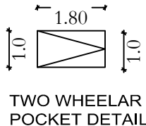
TWO WHEELAR POCKET DETAIL
