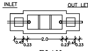
PLAN SEPTIC TANK DETAILS
