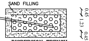
DISPERSION TRENCH
